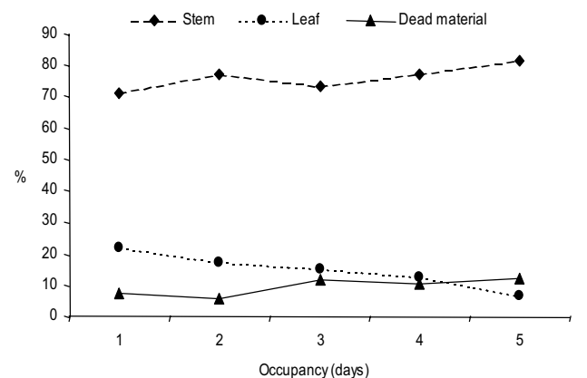
Figure 2. Changes in stem, leaf and dead material composition in bigalta grass per day of occupancy in pasture paddocks
